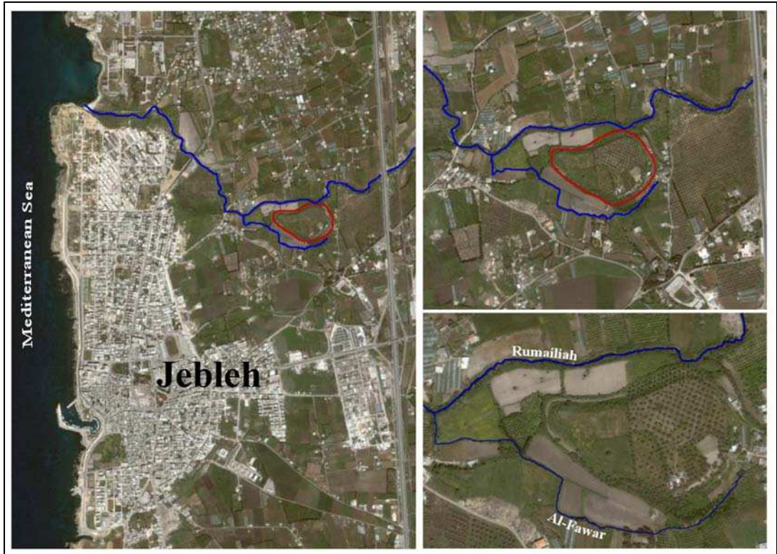
Fig. 1. Satellite image of the Jebleh plain with Tell Tweini (red) and the Rumailiah (N) and Al Fawar (S) rivers. (based on Google Earth™ – 2003)
