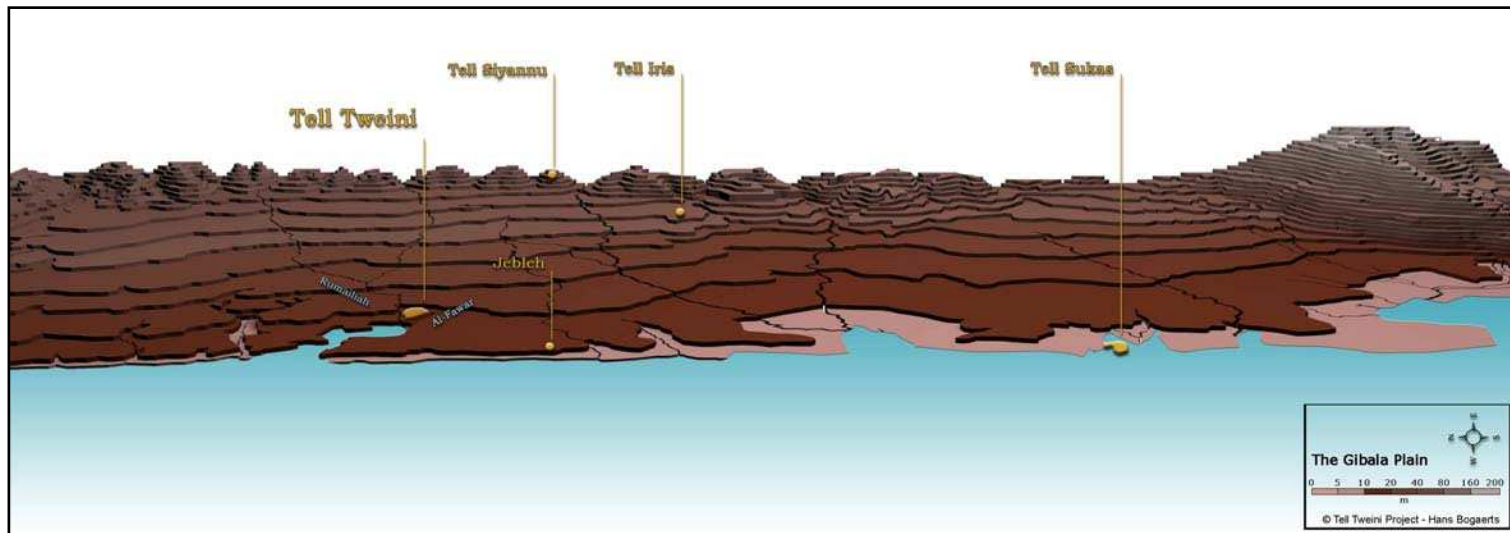
Fig. 3. Sea incursion at Tell Tweini and around Tell Sūkās, after hypothetical 5m rise of relative sea level.
