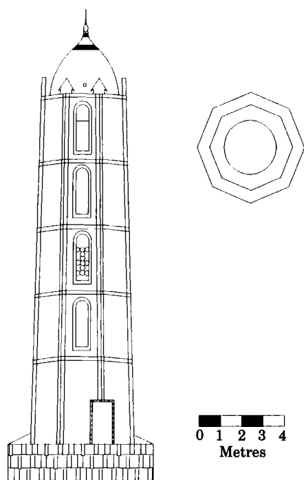
Figure 4. Sketch of the Aden minaret.
