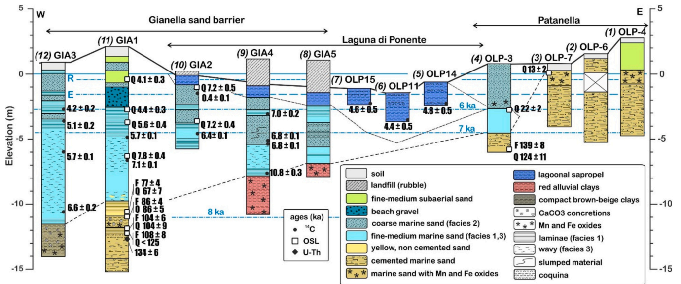
Fig. 4. Distribution of sediment facies and ages along a core transect from the Patanella bank to the Giannella sand barrier. Black long-dashed line: sequence boundary. Black, short-dashed line: base of lagoon layers. Blue dashed lines: sea level at successive 1 kyr time step according to the model of Roy and Peltier (2018). Roman (R) and Etruscan (E) levels from Leoni and Dai Pra (1997). (For interpretation of the references to colour in this figure legend, the reader is referred to the web version of this article.)
