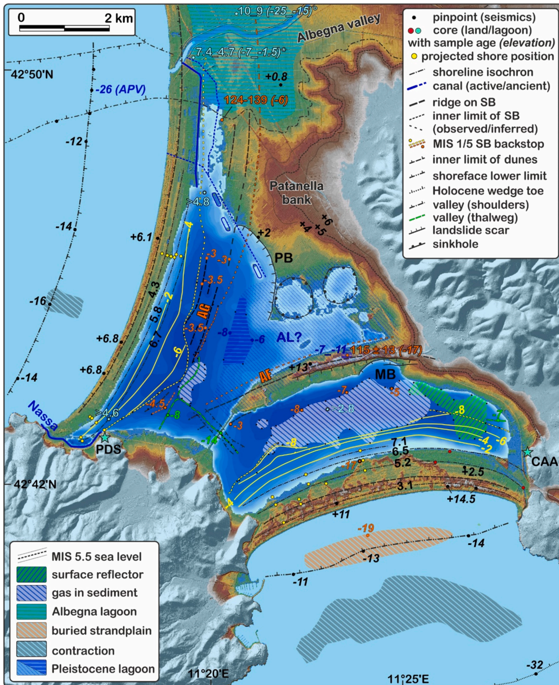
Fig. 9. Map of the tombolo of Orbetello showing morphological features emplaced since the last interglacial. Numbers in italic: elevations amsl in meters (black: modern surface; green: MIS 4–2 paleovalley thalwegs, yellow: contour lines on MIS 1 ridge plain surfaces; orange: MIS 5 surfaces; blue: ancient lagoon layers), other numbers: age in ka of samples dated in this study (with elevation in italic) and of calculated paleoshoreline positions. Earlier published ages from: ° ( Mazzini et al., 1999 ), * ( Chapkanski et al., 2022 ). AG: ancient Giannella, AF: Albegna Feniglia, AL?: putative ancient lagoon, APV: Albegna paleovalley, CAA: Cosa-Ansedonia aquifer, MB: La Madonnella Bight; PB: Patanella Bight; PDS: Punta degli Stretti cave. (For interpretation of the references to colour in this figure legend, the reader is referred to the web version of this article.)
