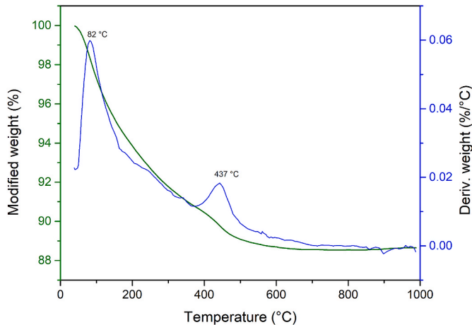
Fig. 3. TGA curve (green) and Derivative thermogravimetry (DTG) curve (blue) of a Trajan sample (TRA8). (For interpretation of the references to colour in this figure legend, the reader is referred to the Web version of this article.)
